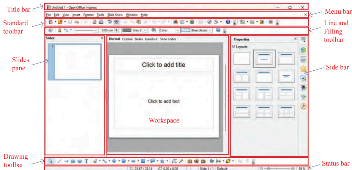
Fig. 16.2: Components of Impress Window
