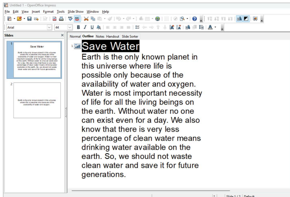
Fig. 17.15: Outline View
