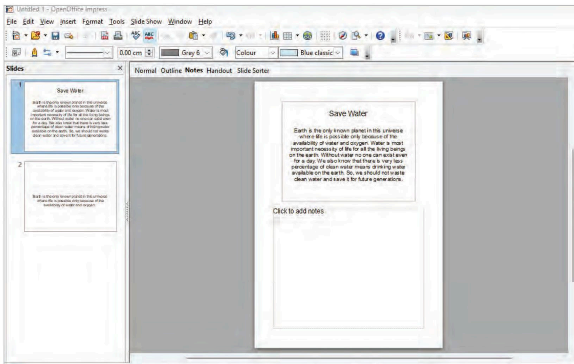
Fig. 17.17: Notes View
