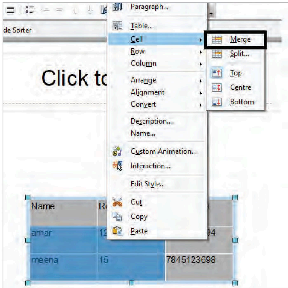
Fig. 19.9: Merging Cells
