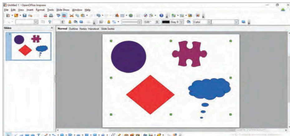
Fig. 20.10: Grouping Shapes
