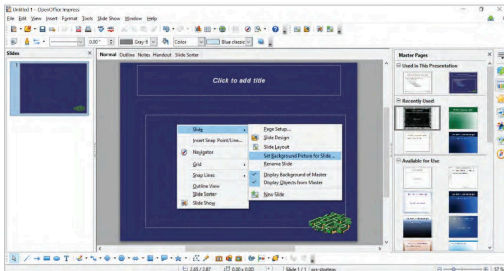
Fig. 21.6: Saving Background
