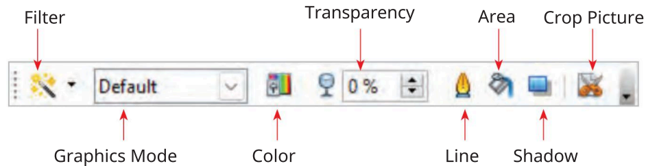
Fig. 20.6: Picture Toolbar
