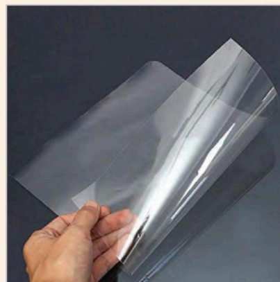
Fig. 15.2: Transparency
