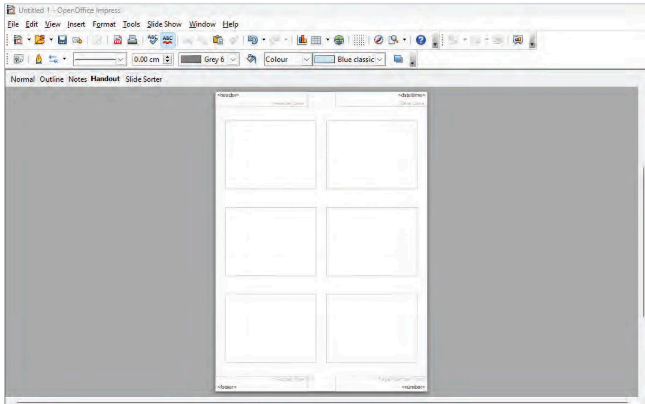
Fig. 17.18: Handout View
