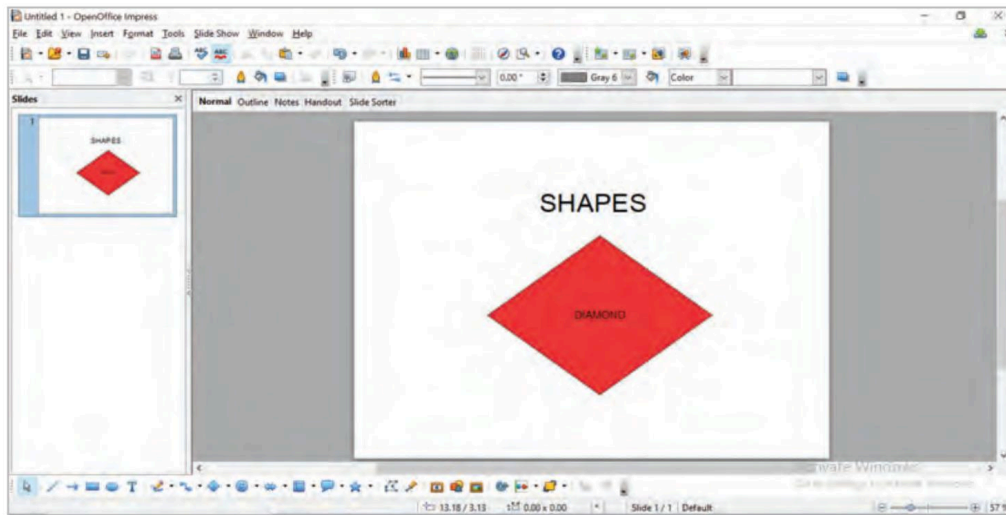
Fig. 20.9: Adding Shapes
