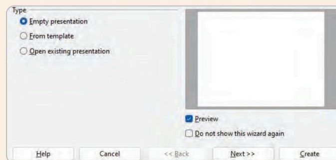
Fig. 16.1: Presentation Wizard
