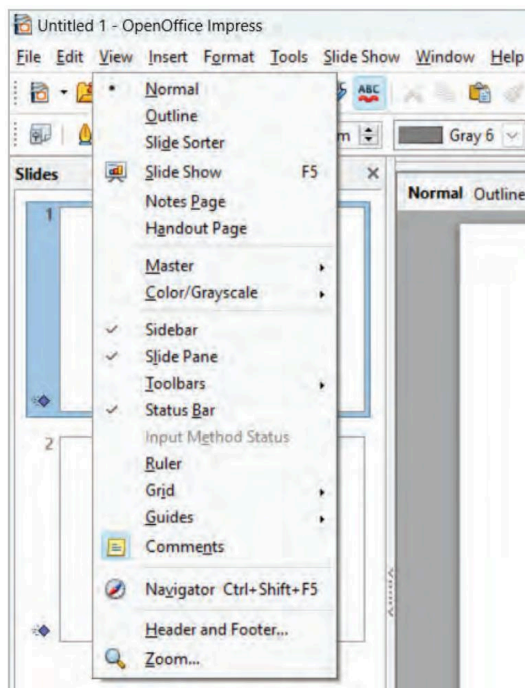
Fig. 17.13: Selecting Views
