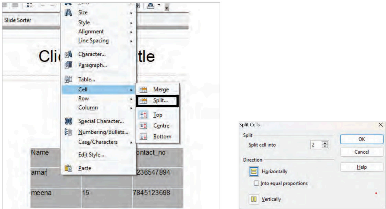
Fig. 19.10: Splitting Cell
