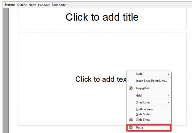
Fig. 17.11: Pasting Content
