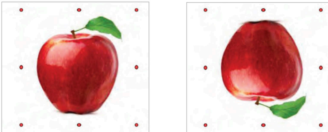
Fig. 20.3: Rotating Images
