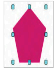
Fig. 20.11: Resizing Shape
