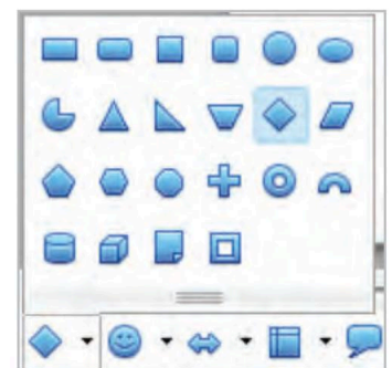
Fig. 20.8: Basic Shapes
