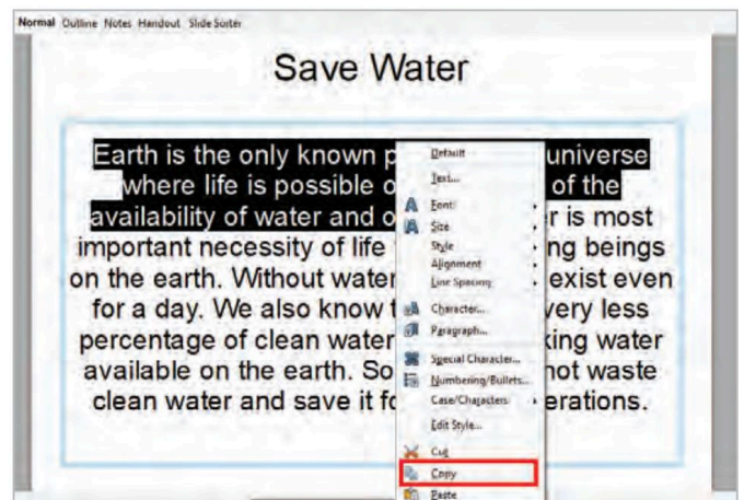
Fig. 17.10: Copying Content
