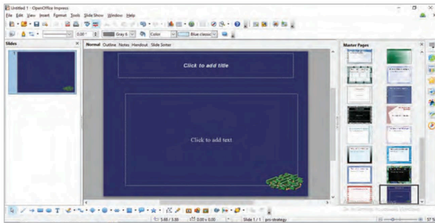
Fig. 21.4: Applying Theme
