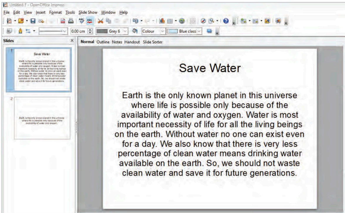
Fig. 17.14: Normal View
