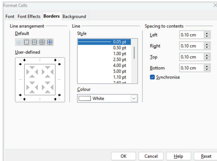
Fig 19.11: Borders Tab
